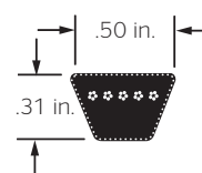
A Section
