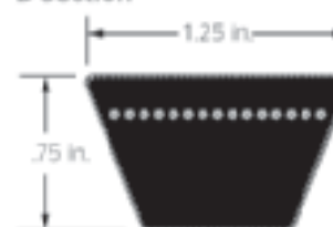
D Section
