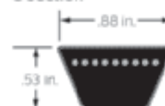
C Section
