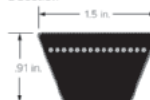
E Section
